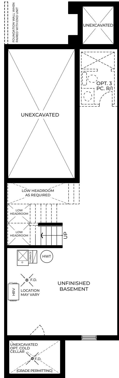
BASEMENT PLAN ELEV. A1
