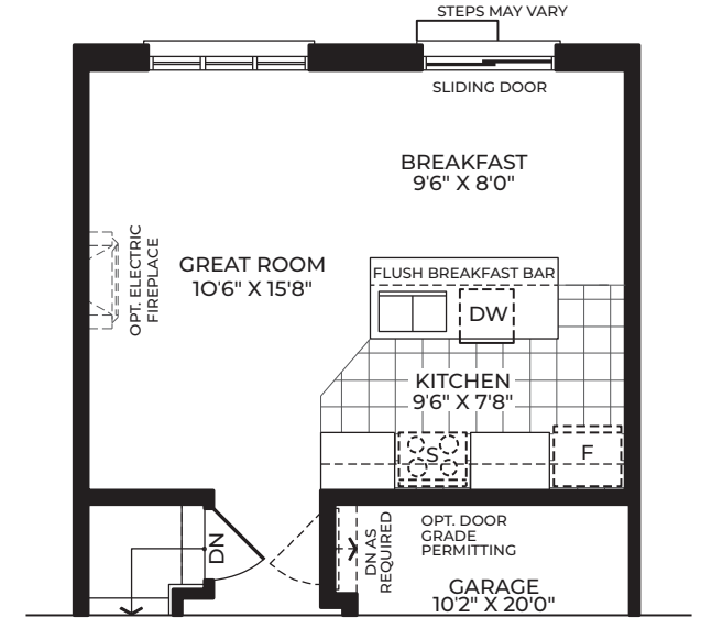
PARTIAL ALT. MAIN FLOOR PLAN ELEV. B
