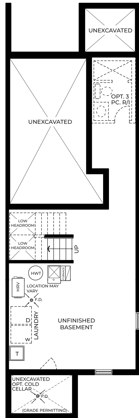
BASEMENT PLAN ELEV. B2 END
