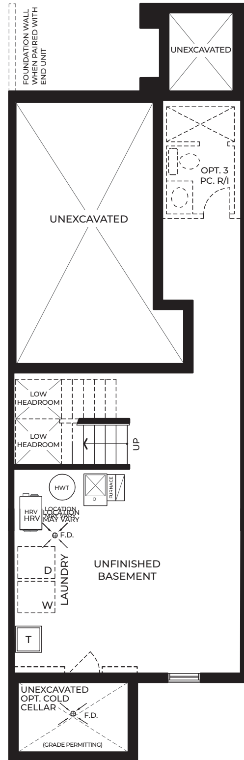
BASEMENT PLAN ELEV. A2
