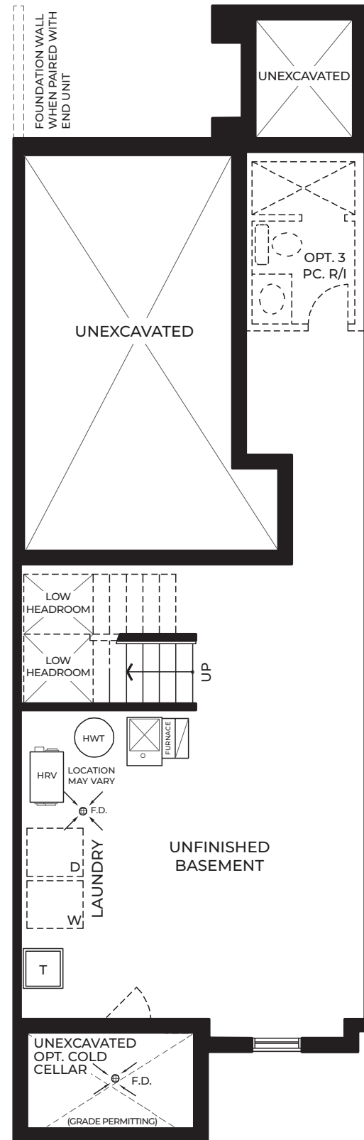
BASEMENT PLAN ELEV. A1
